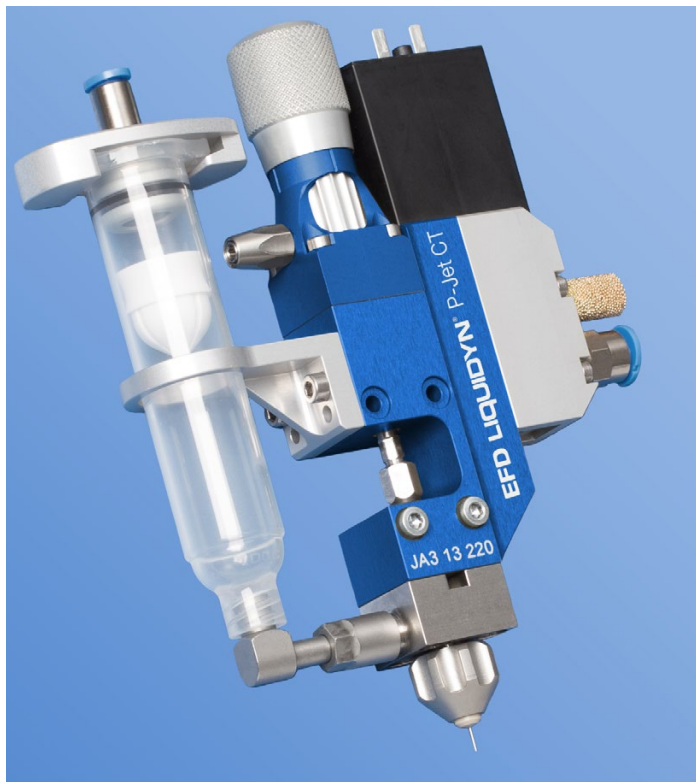
The high-performance Liquidyn P-Jet CT valve provides both non-contact and contact dispensing capability.
