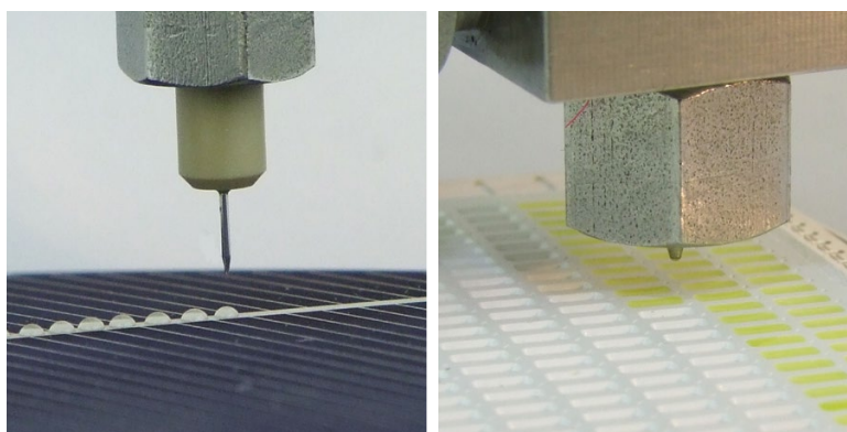
Non-contact micro-dispensing of beads and fills onto delicate surfaces is easy and repeatable.
